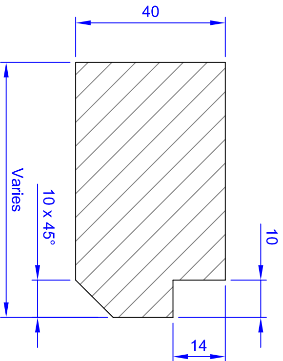
Section B-B (Varies)
